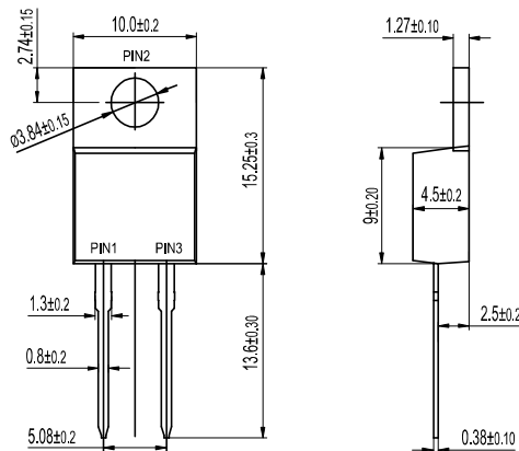
TO-220AC DR10XX
